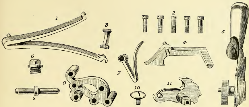
Pieces of Modern Hammer Gun-lock.
